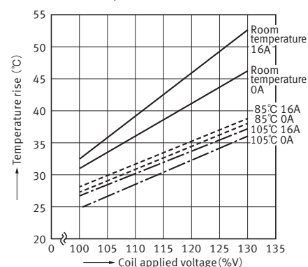
2. Coil temperature characteristics ( Average )
