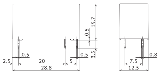
External dimensions
