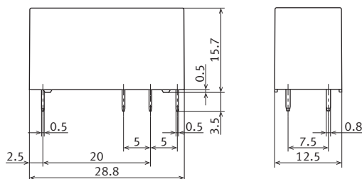
External dimensions
