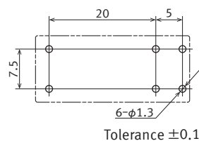
Recommended PC board pattern ( BOTTOM VIEW )
