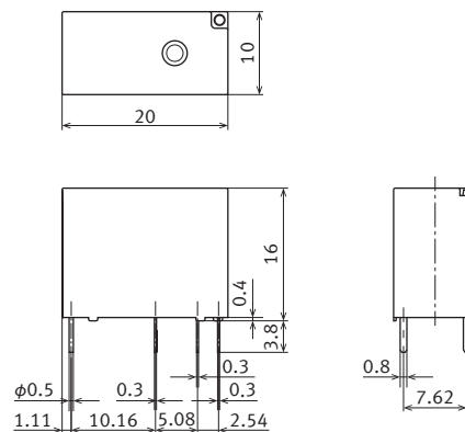
External dimensions
