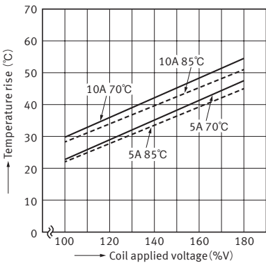
2-1. Coil temperature characteristics ( Standard type, Inrush/reinforced insulation type: 1 Form A )
