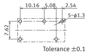
Recommended PC board pattern ( BOTTOM VIEW )
