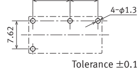
Recommended PC board pattern ( BOTTOM VIEW )
