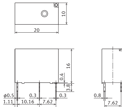
External dimensions
