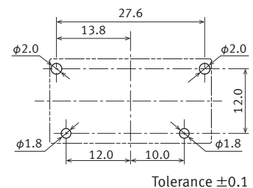
Recommended PC board pattern ( BOTTOM VIEW )
