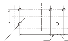
Recommended PC board pattern ( BOTTOM VIEW )
