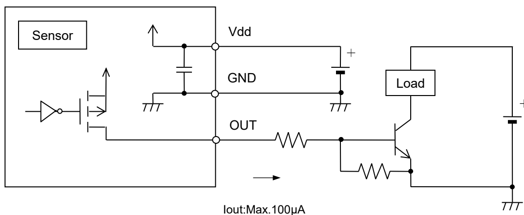
4-4 Wiring Diagram
