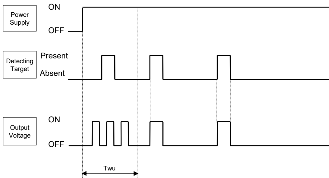
4-3 Timing Chart
