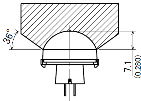
Detection range
