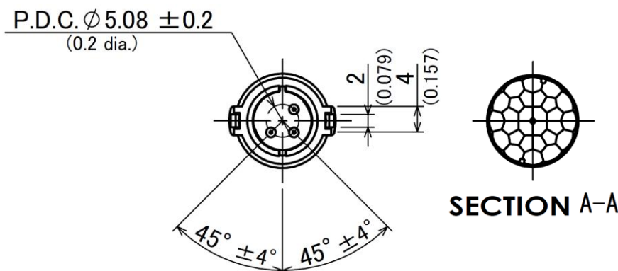
Bottom VIEW
