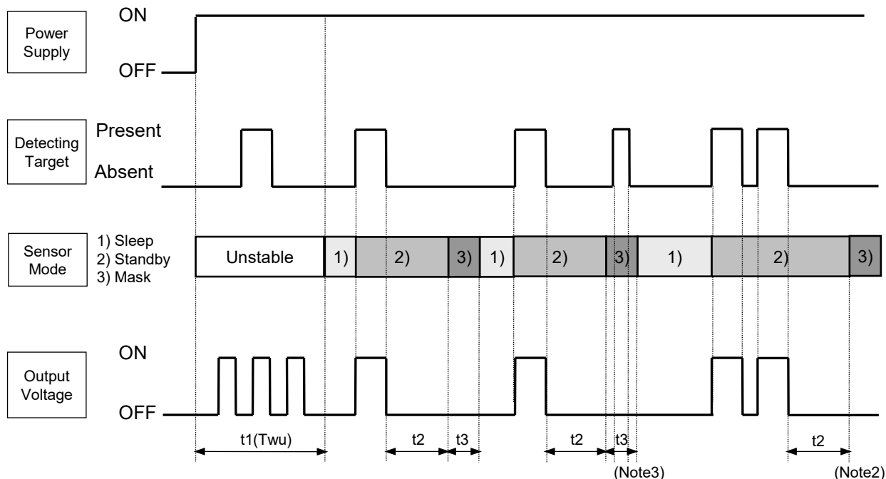
4-4 Timing Chart
