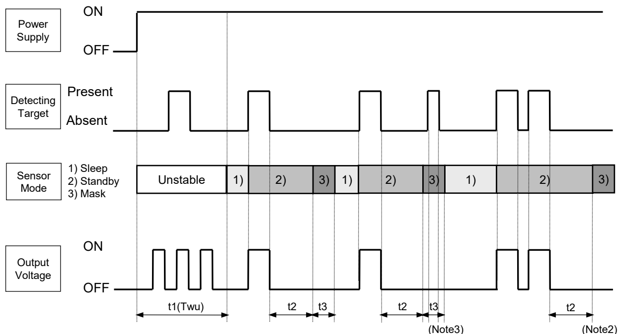
4-4 Timing Chart
