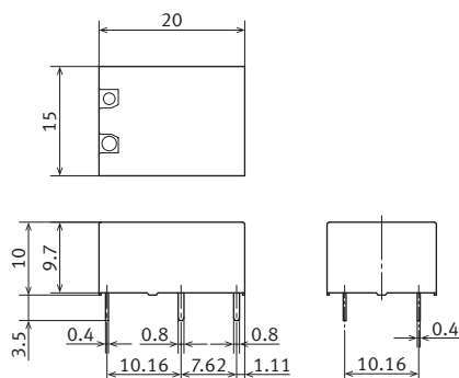
External dimensions
