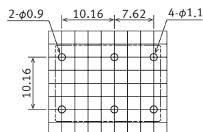
Recommended PC board pattern ( BOTTOM VIEW )
