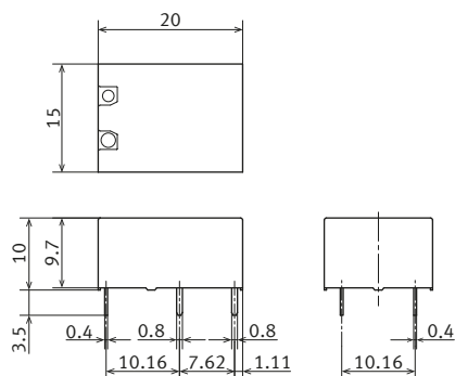
External dimensions
