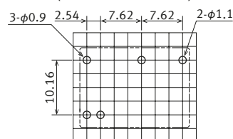
Recommended PC board pattern ( BOTTOM VIEW )
