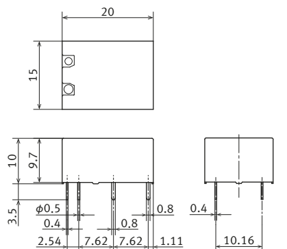
External dimensions
