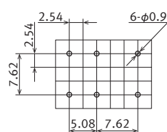
2 coil latching
