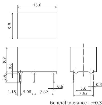
External dimensions
