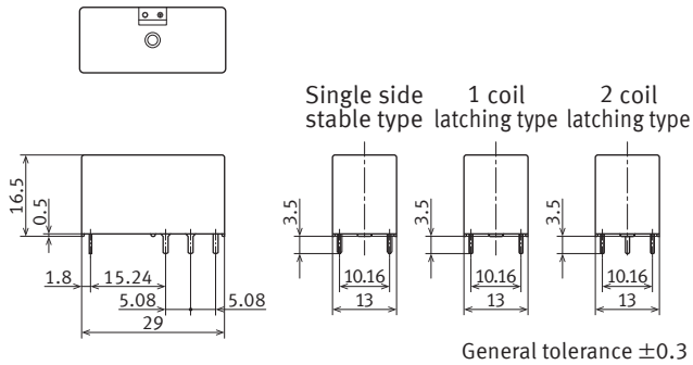
External dimensions
