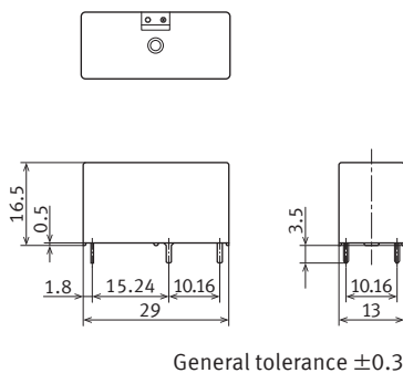
External dimensions
