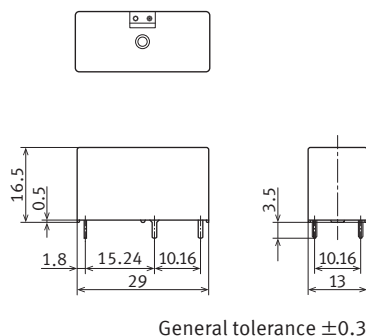
External dimensions
