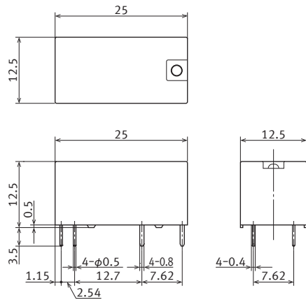
External dimensions
