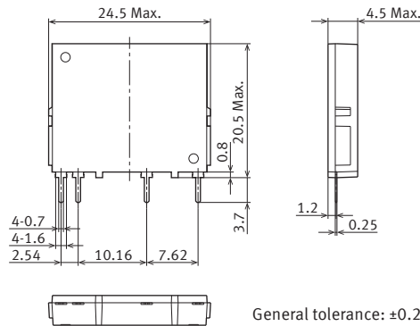
External dimensions
