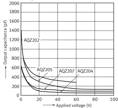
18-2. Output capacitance vs. applied voltage characteristics ( AC/DC type )
