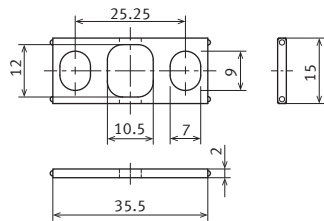
External dimensions
