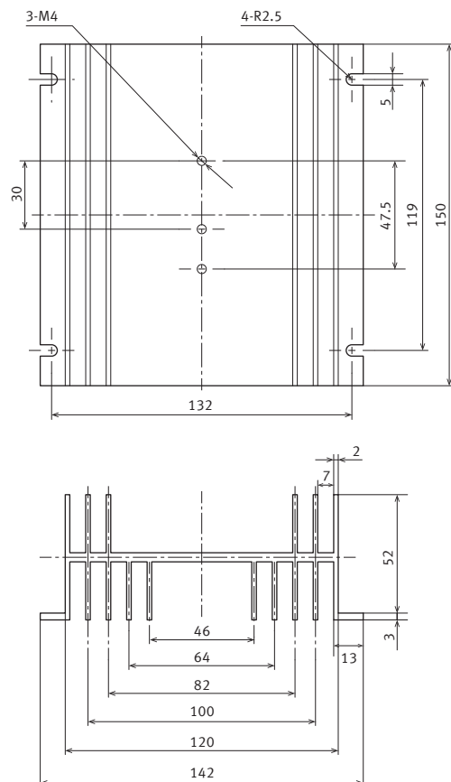
External dimensions
