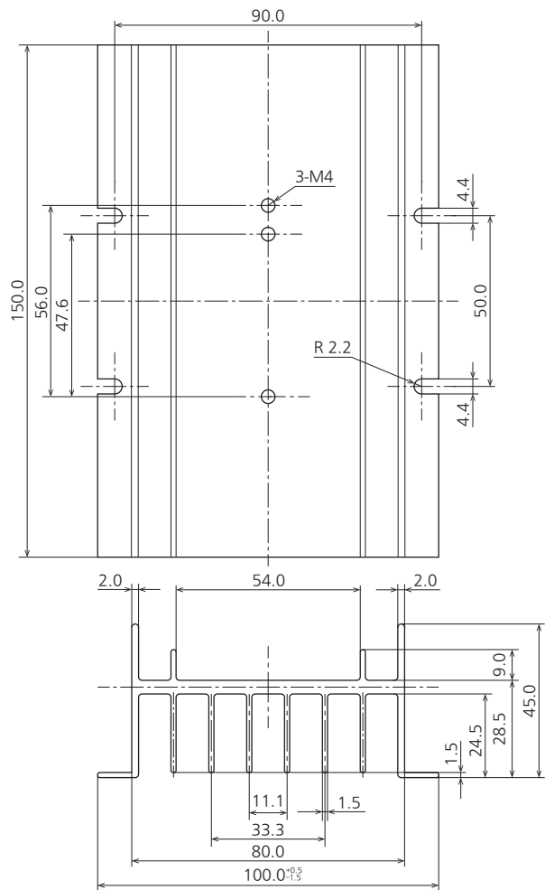
External dimensions
