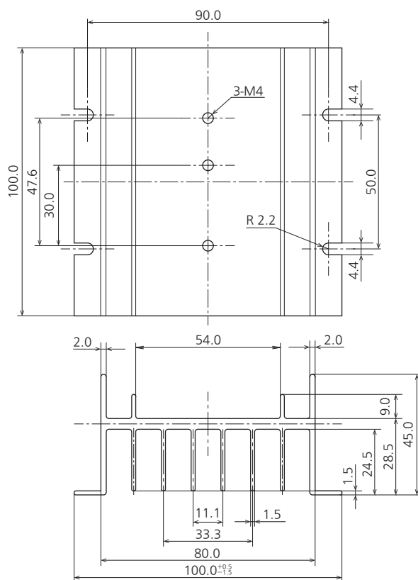
External dimensions
