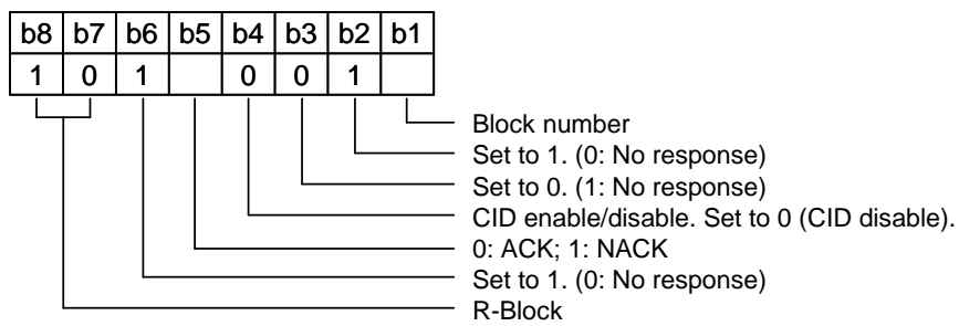
Figure 4-17 R-block Coding
