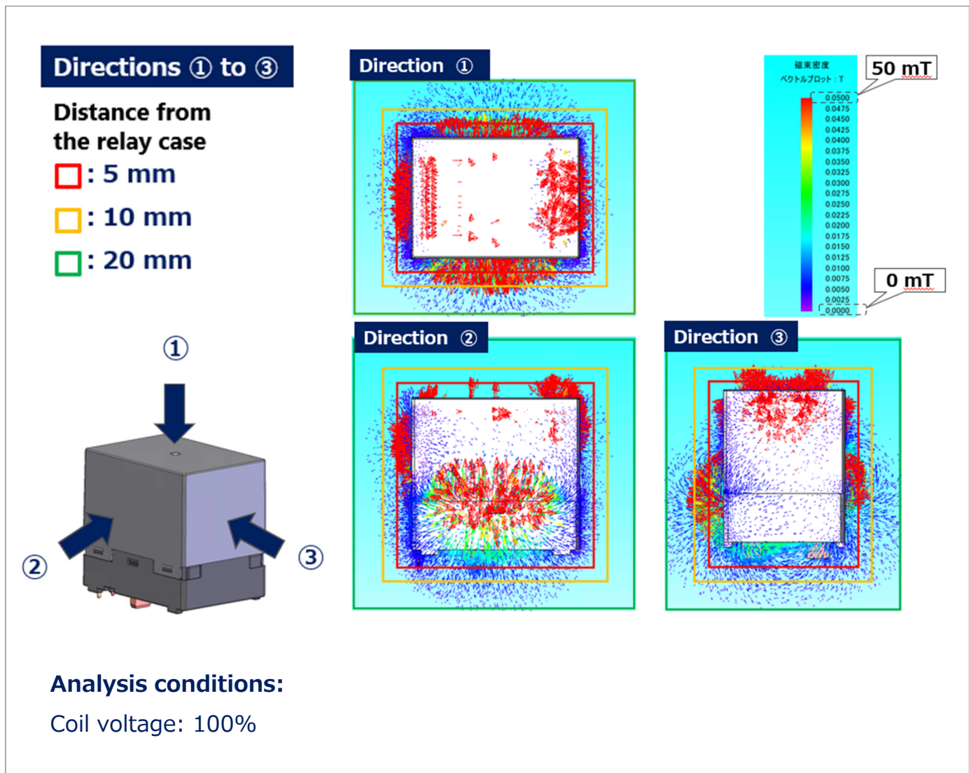
[Figure 13: Magnetic field analysis data (reference data)]
