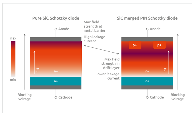
Figure 4: Adding P-wells to a SiC Schottky diode displaces the area of maximum field strength under reverse bias, away from the anode metal.
