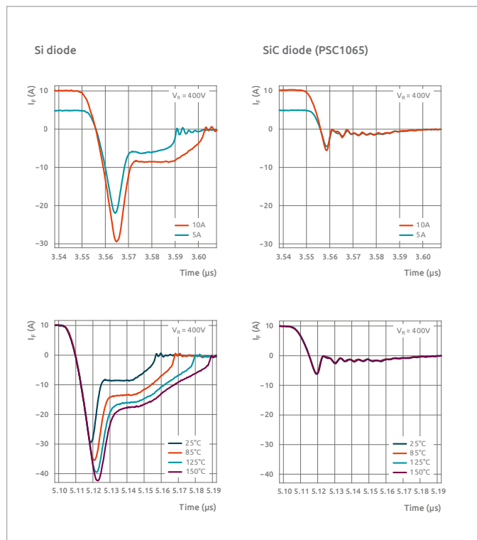
Figure 6: Comparison of reverse recovery behaviour of Si and SiC under various operational conditions.
