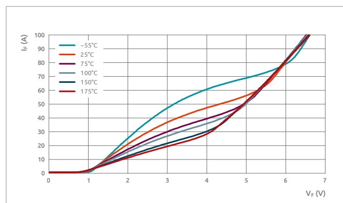
Figure 5: Static I-V behaviour of SiC MPS diodes, including overcurrent.
