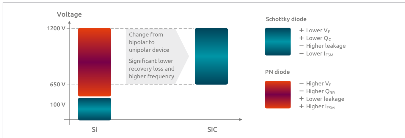
Figure 2: Comparison of Si and SiC power diodes vs blocking voltage.
