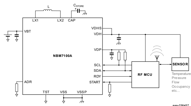
Fig. 2. Simplified Application
