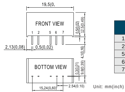
▲ MDD01 0.77" x 0.39" x 0.49"
