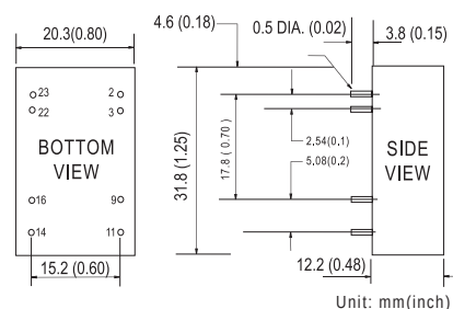
▲ DCW05 1.25" x 0.80" x 0.48"
