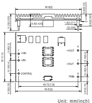
▲ NSD15-S 2" x 1.5" x 0.387"
