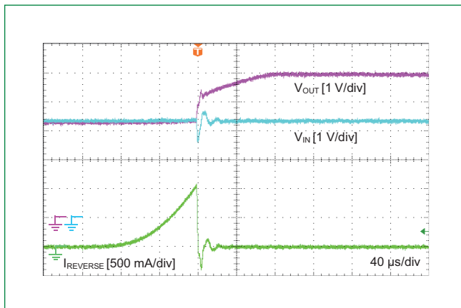
Figure 15 - Reverse Current Blocking at Switch On V_{IN} = Open, C_{IN} = 1.0\mu F , C_{OUT} = 0.1\mu F
