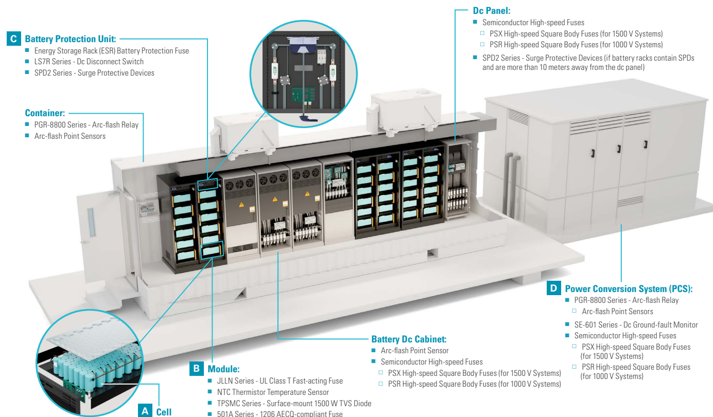
FIGURE 1. A battery energy storage system (BESS).
