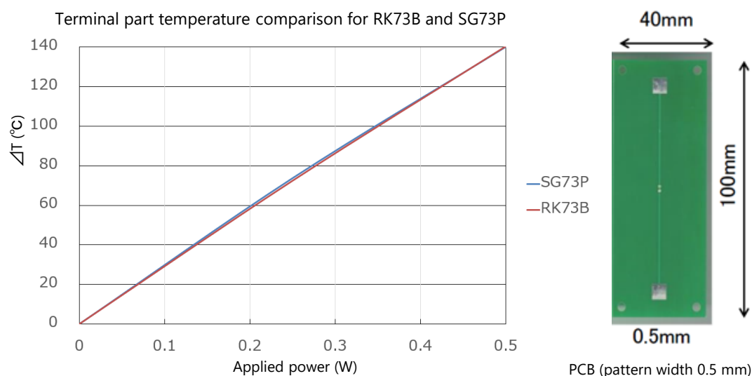
Figure 1 Applied power and temperature rise
