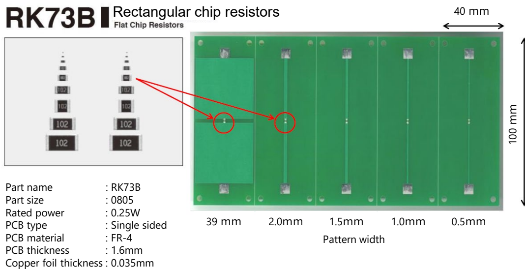
Figure 2 Information on PCB and resistors used
