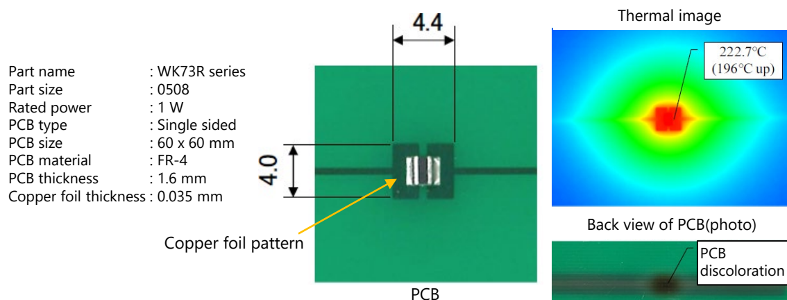
Figure 4 Temperature rise without appropriate heat dissipation design
