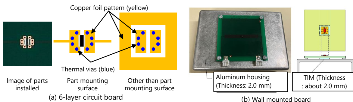
Figure 5 Example of heat dissipation design
