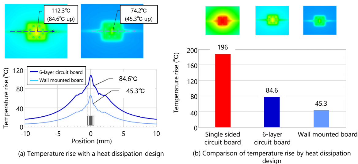
Figure 6 Effect of heat dissipation design
