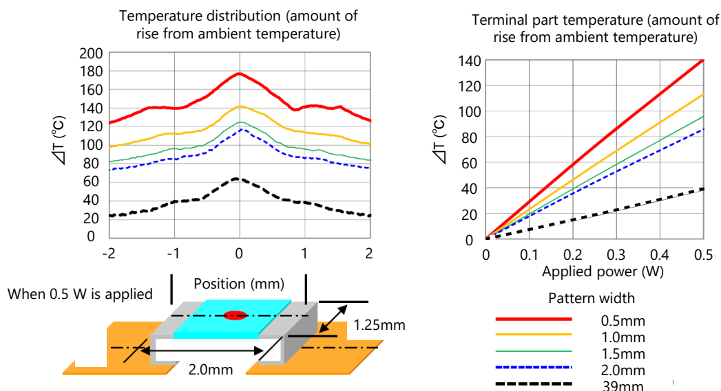
Figure 3 Relationship between pattern width and temperature rise
