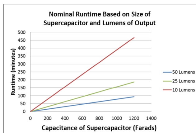
Figure 2: Runtime vs. capacitance for different LED lumen outputs. This assumes that the supercapacitor is rated to 2.7 V and discharged to 1.35 V, an LED efficiency of 100 lumens per watt and a driver (power supply) efficiency of 85%.
