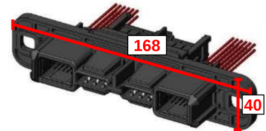
Plug
