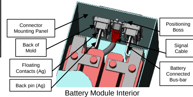
Battery Module Interior
