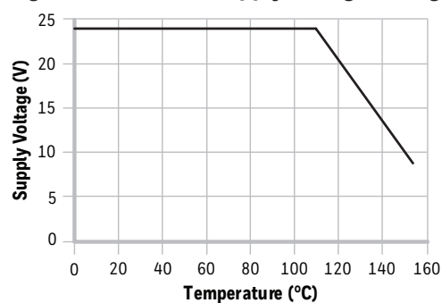
Figure 1. Maximum Supply Voltage Rating
