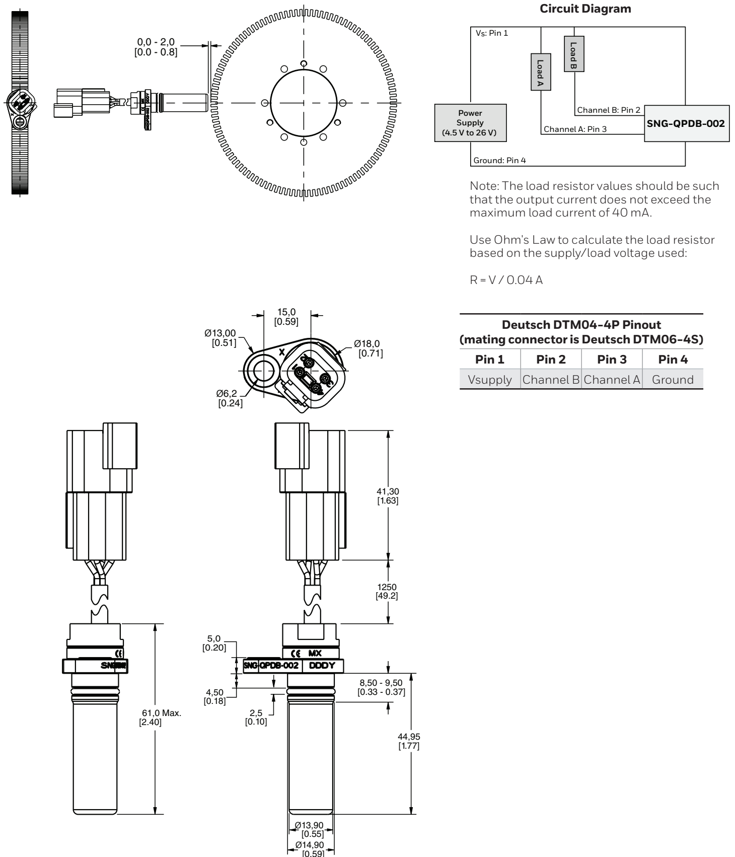
Figure 9. SNG-QPDB-002 Mounting Dimensions (For reference only: mm/[in].)
