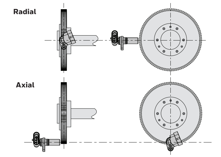
Figure 3. Possible Mounting Orientations
