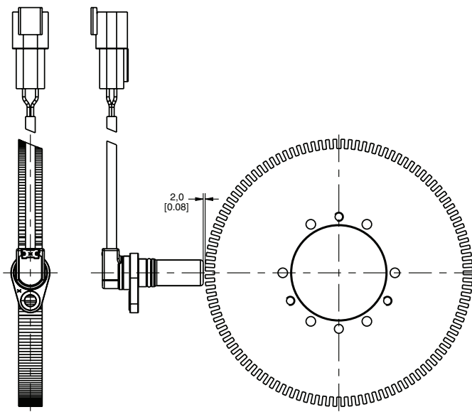
Figure 5. SNG-QPCA-001 Mounting Dimensions (For reference only: mm/[in].)
