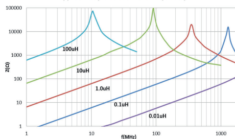
Typical Impedance vs. Frequency
