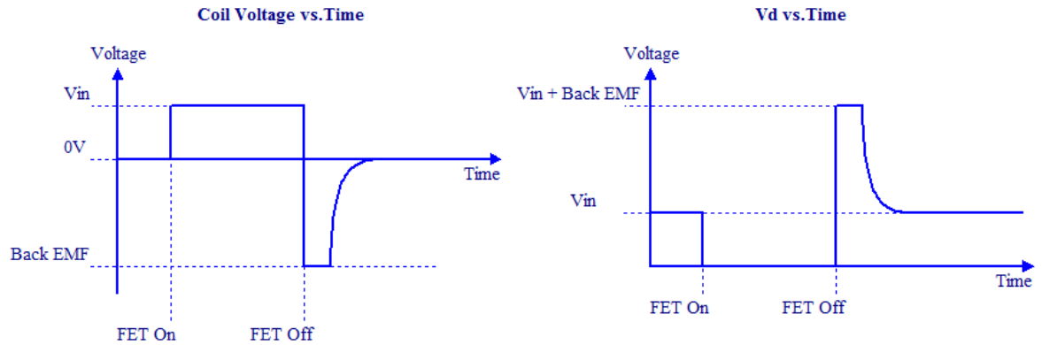
Figure 6. Coil Voltage and V_d vs. Time
