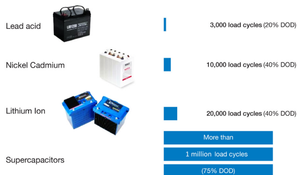
Figure 1: Comparing cycling capabilities of Lead acid, Nickel Cadmium, Lithium ion, and supercapacitors storage technologies
