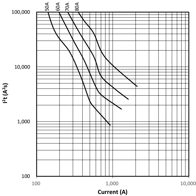
I 2 t vs. current curve
