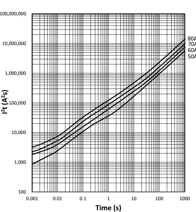
I²t vs. time curve
