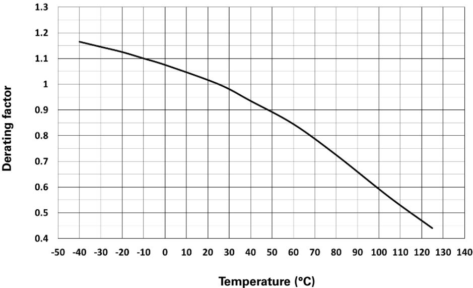
Temperature derating curve
