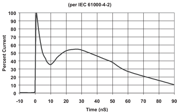
Figure 1. IEC 61000-4-2 ESD pulse
