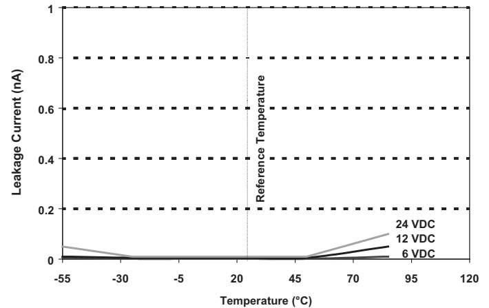
Figure 7 Average off state current leakage vs. temperature
