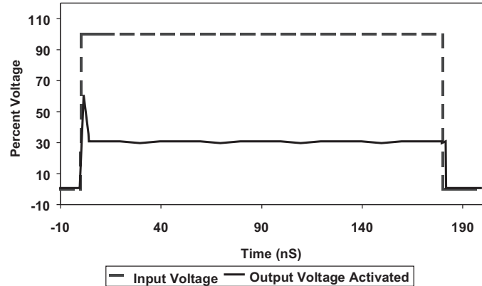
Figure 2. Transmission Line Pulse
