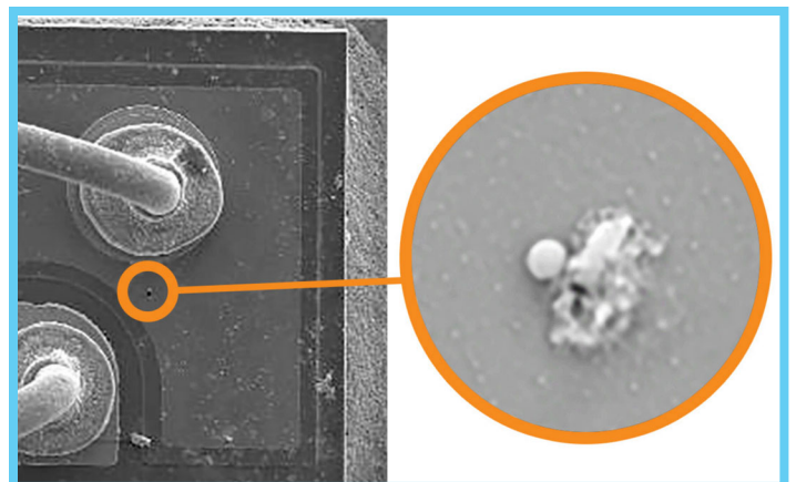
Figure 1. Typical ESD Damage 7
