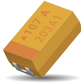
Fig. 2. The KYOCERA AVX TBJ series SRC8000 COTS-Plus space-level tantalum capacitors are currently available in six case sizes spanning EIA metrics 3216-18 to 7361-43 with ratings spanning 6 to 50 V and 0.10 to 680 \mu F.
