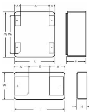
Undertab Termination
