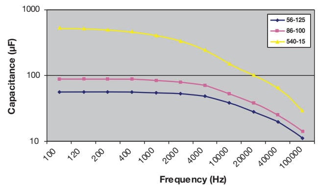
Figure 1.1.4 a: TWC Typical Capacitance vs. Frequency
