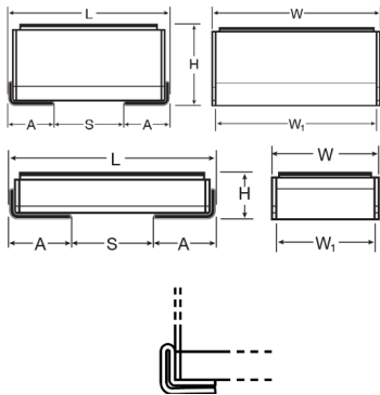
'J' Lead Termination (flex)
