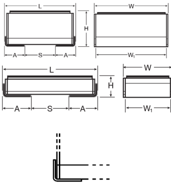
'J' Lead Termination (L-shape)
