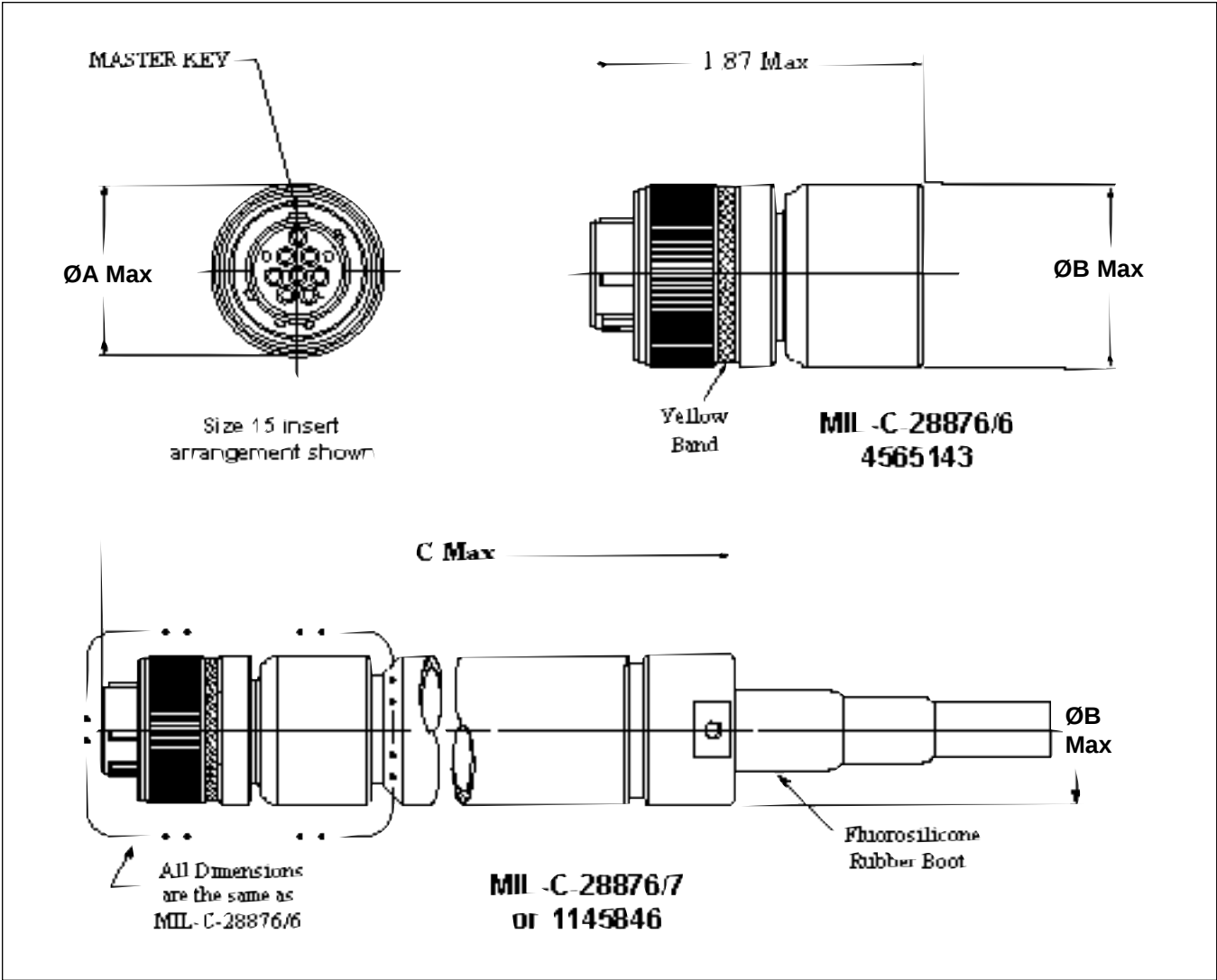
Dimension Table, Plug Connector
