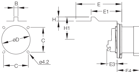
Dimensions (mm)
