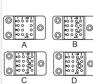
Socket Configurations
