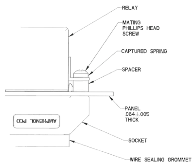
Mounting Hardware
