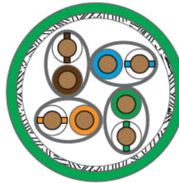
S/FTP
