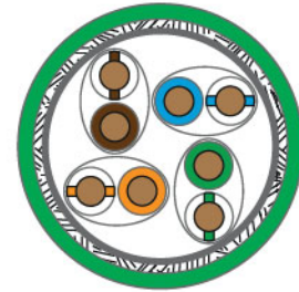
SF/UTP
