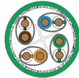
S/FTP with cross element
