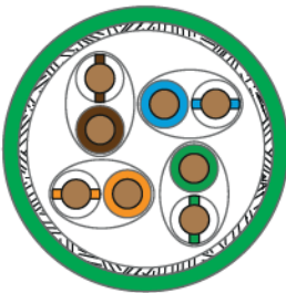
S/UTP
