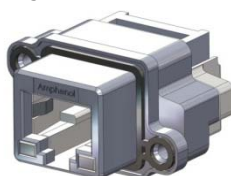
MRJR-538X-01 SHOWN RIGHT ANGLE, PCB TAIL, 8 POSITION RJ45
