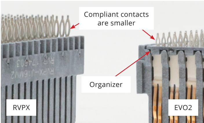
Figure 2 - Backplanes
