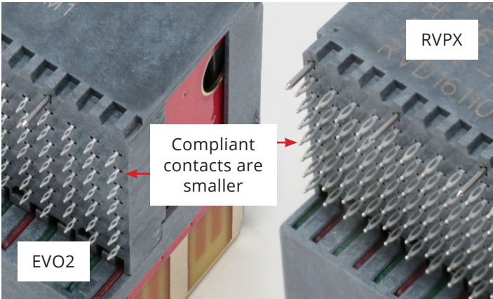
Figure 1 - Daughtercards
