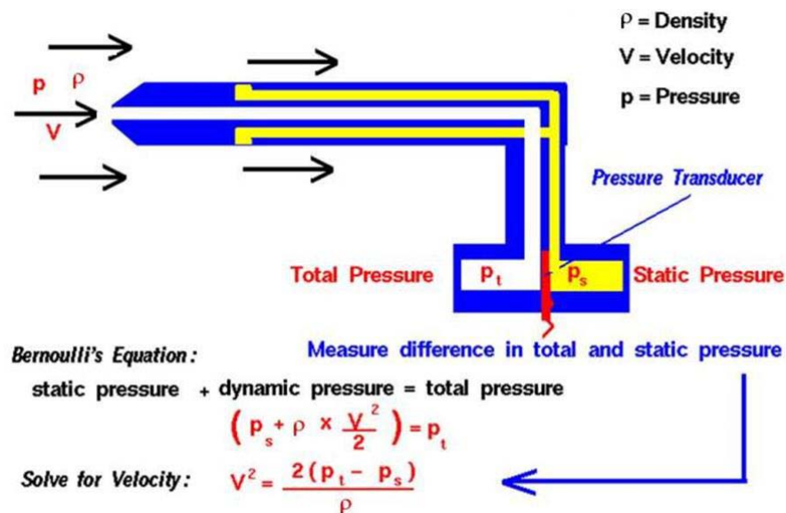
Figure 2. A Pitot-static or Prandtl tube used to measure aircraft velocity.
