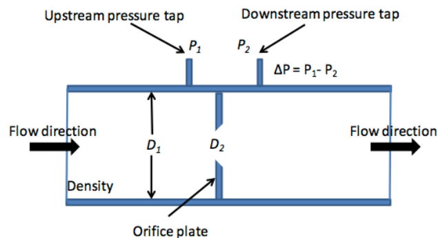
Figure 1. Elements of a \Delta P flow measurement.
