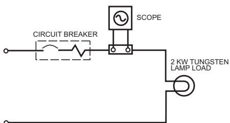
Fig. 14 Transient current from a tungsten lamp load.
