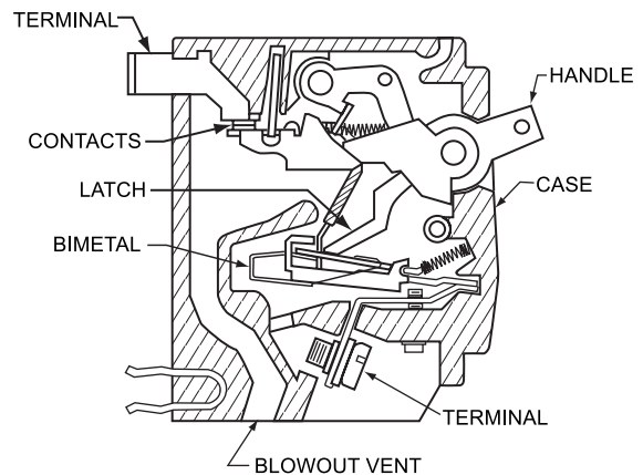
Diagram of a standard thermal circuit breaker
