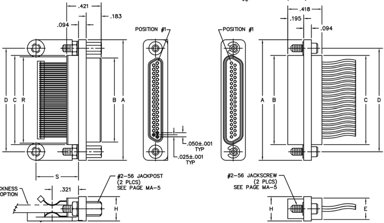
PLUG
