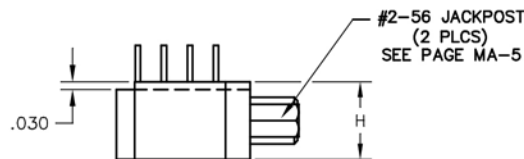
(PLUG SHOWN)
