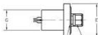
#2-56 LOCKING HELICAL THREAD INSERT* (2 PLCS) #2-56 REAR PANEL MOUNT JACKPOST (2 PLCS)
