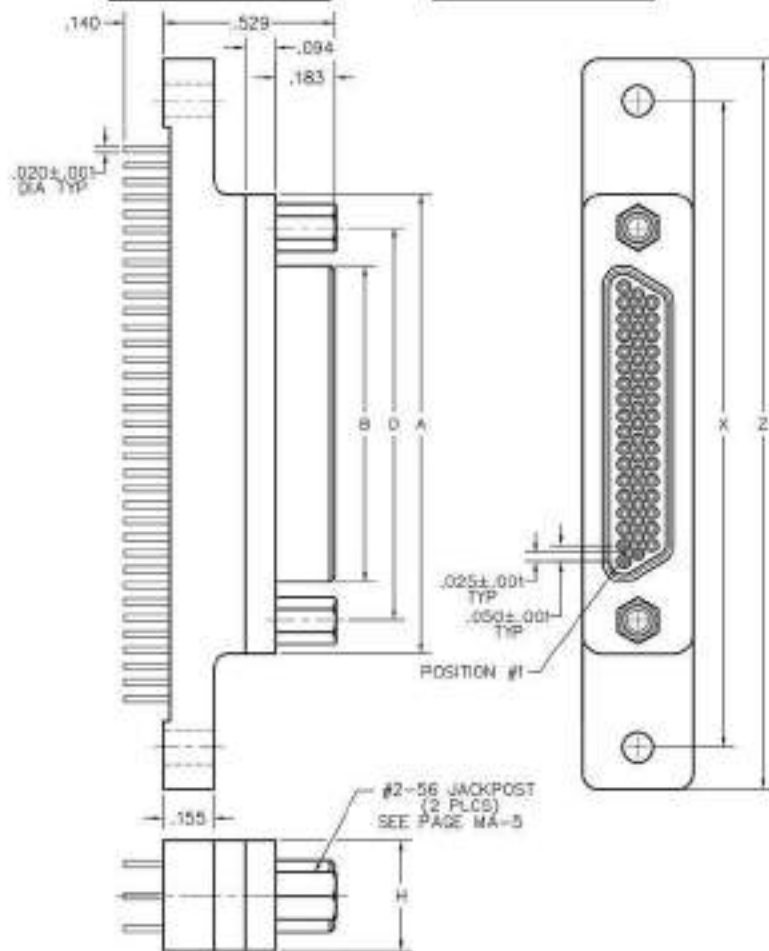
PLUG
