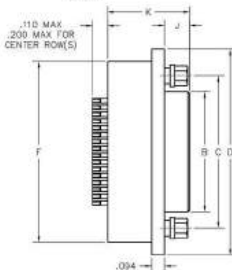
MM-2E2-031-161-25WA (PLUG)
