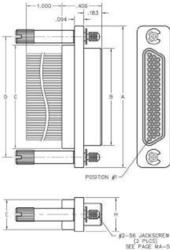
PLUG
