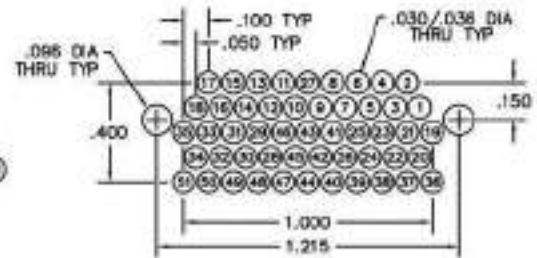
RECEPTACLE PC BOARD LAYOUT COMPONENT SIDE
