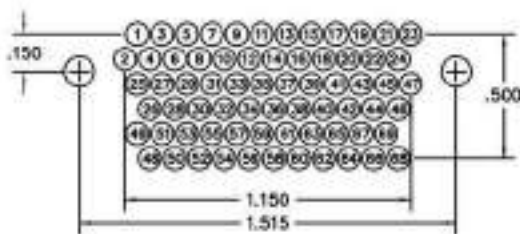
** 69 POSITION
