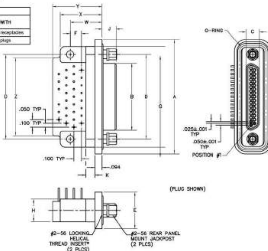
MK-202-031-335-2605 (PLUG)
