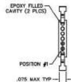
TERMINATION VIEW
