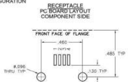
FOOTPRINT/PAD CONFIGURATION
