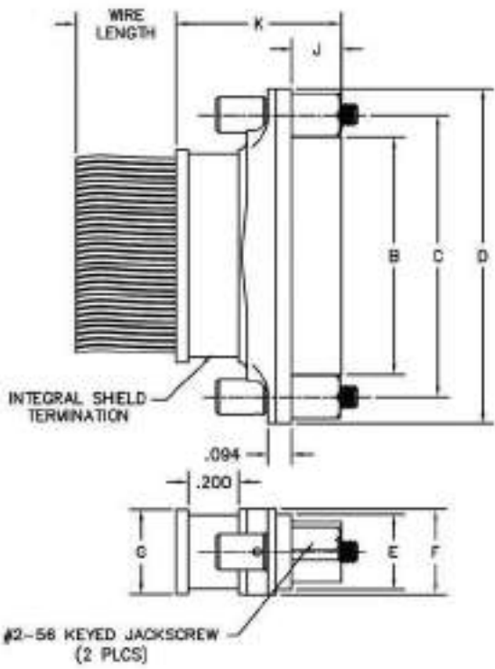
MM-2P2-031-101-44WA (PLUG)
