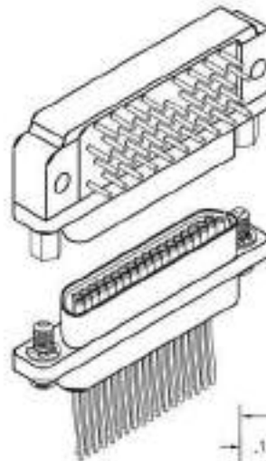
MQHT-222-037-261-41WS (METAL)
