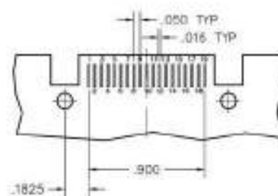
RECEPTACLE PC BOARD LAYOUT CIRCUIT SIDE
