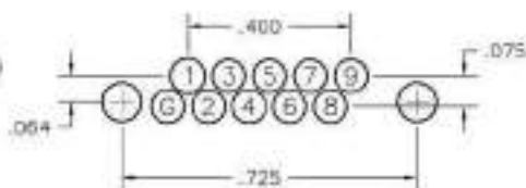
9 POSITION
