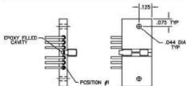
TERMINATION VIEW
