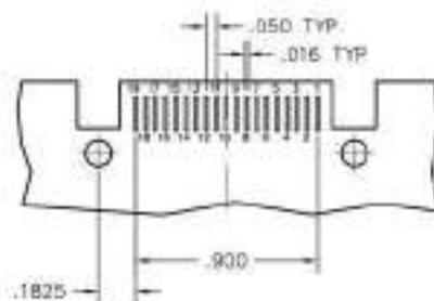
PLUG PC BOARD LAYOUT CIRCUIT SIDE
