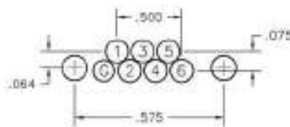
6 POSITION
