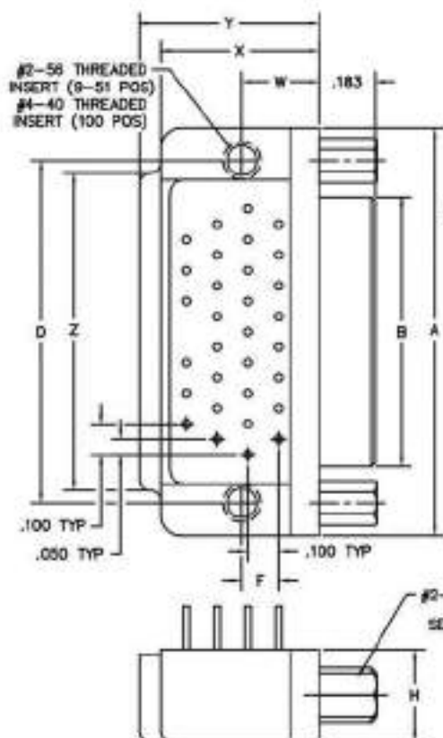
PLUG
