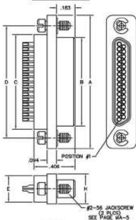
PLUG
