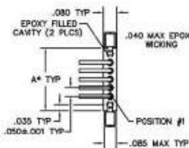
TERMINATION VIEW
