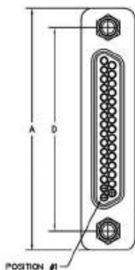
PLUG
