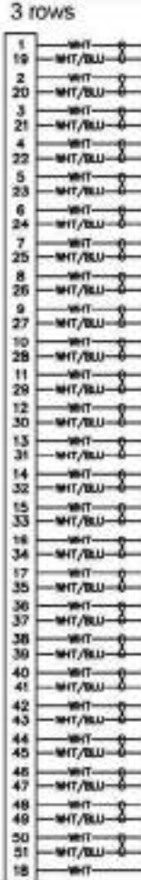
51 POSITION 3 rows
