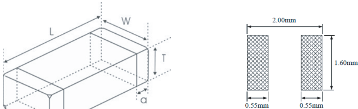
Dimension: mm
